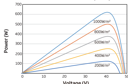
P-V CURVES OF PV MODULE (610W)
